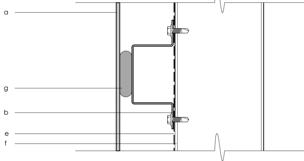
Mid Panel Detail
