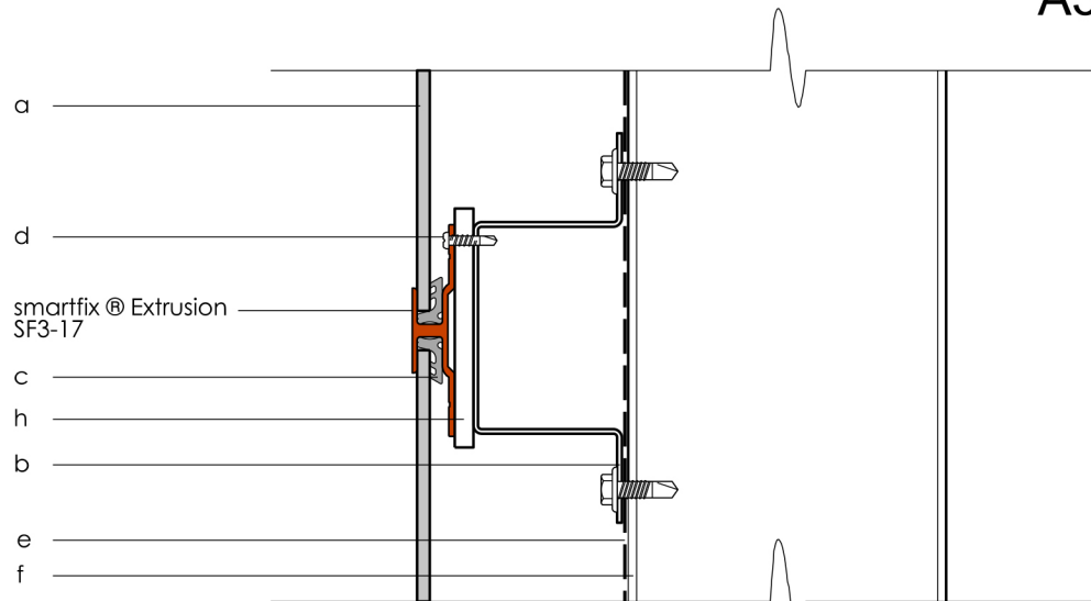
Horizontal Panel Joint Detail
