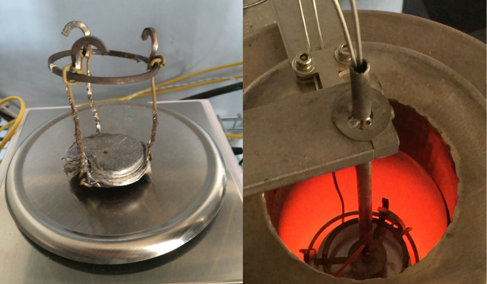
SOLIDAL® AS1530.1 TESTING SOLIDAL® is rigorously tested to ensure maximum Building Safety.
