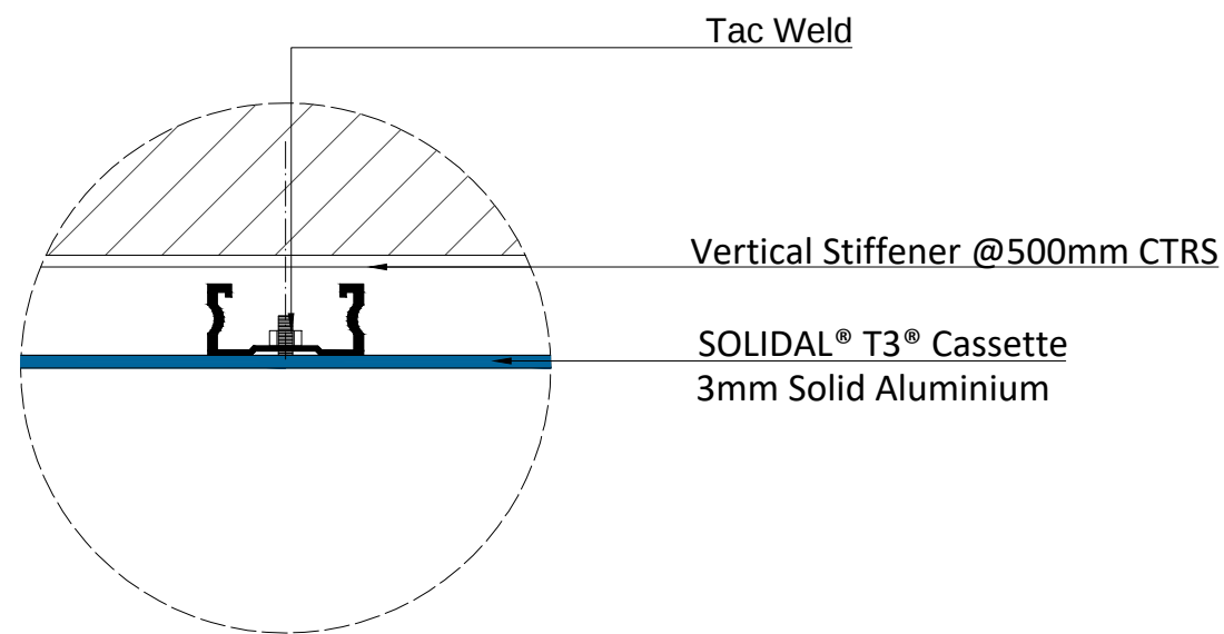
OPTION 1: Stiffeners with tac-welds
