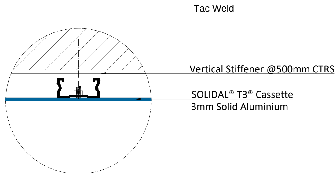
OPTION 1: Stiffeners with tac-welds
