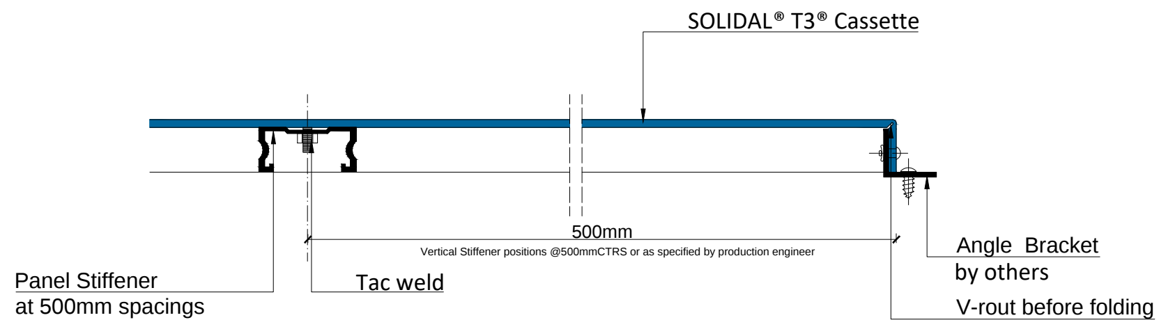
1 - SECTIONAL PLAN VIEW showing Vertical Stiffener and folded corner
