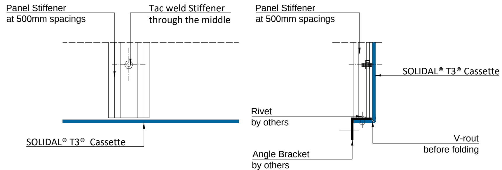
2 - INSIDE VIEW showing Vertical Stiffener
