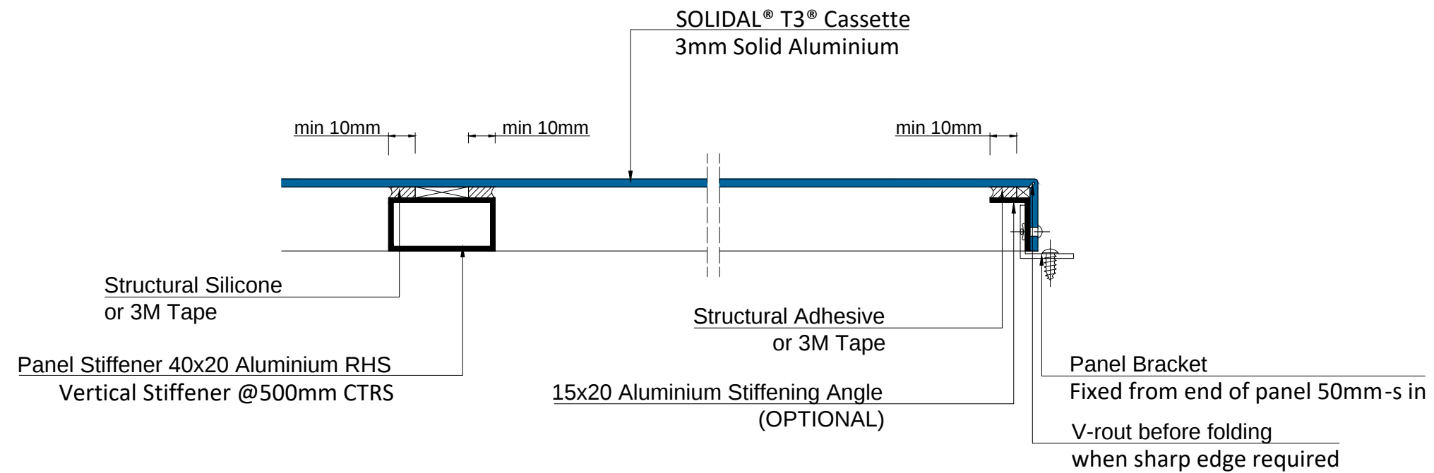
1 - SECTIONAL PLAN VIEW showing Vertical Stiffener
