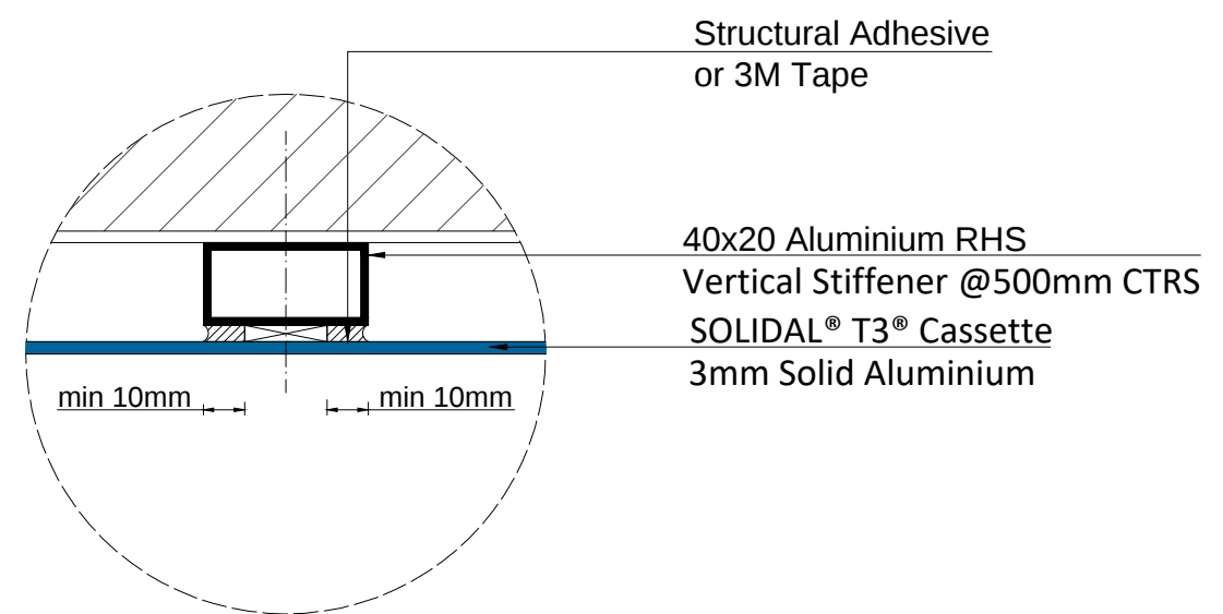
OPTION 2: Stiffeners with structural adhesive
