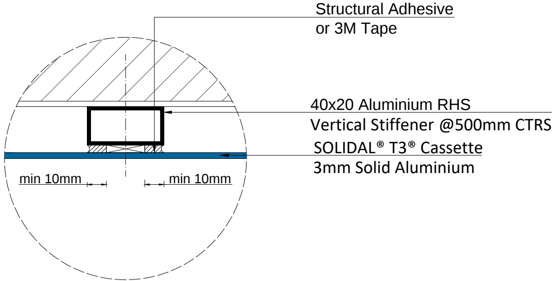
OPTION 2: Stiffeners with structural adhesive
