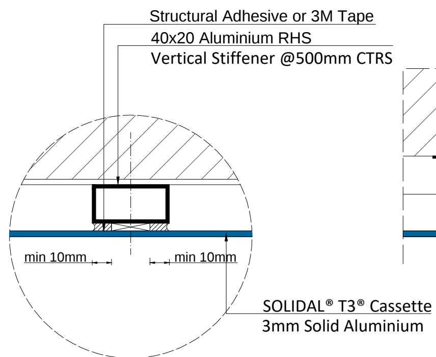
OPTION 2: Stiffeners with structural adhesive
